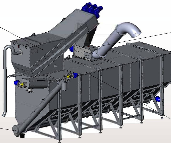
Jagged multi-screw with SINT® screen
